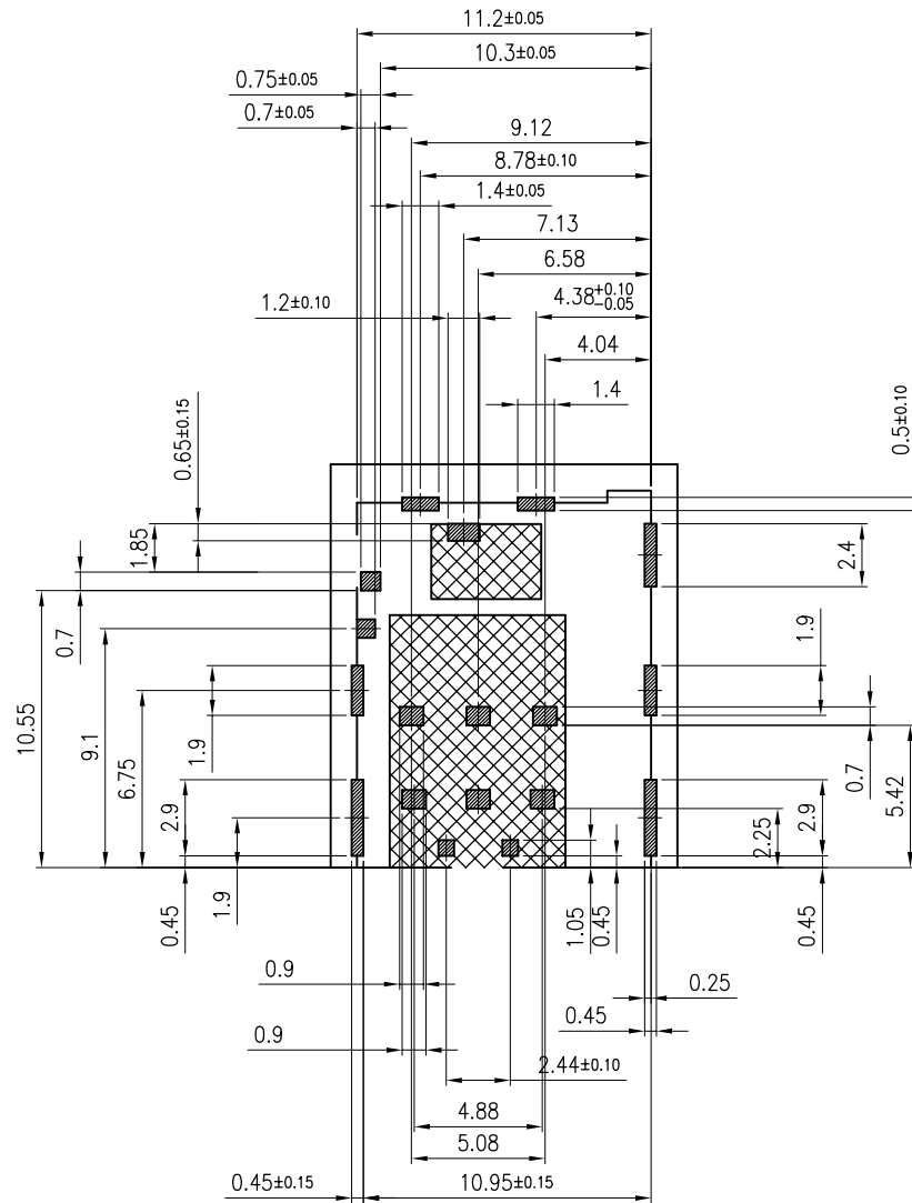
RECOMMENDED PCB LAYOUT TOP VIEW (TOLERANCE:±0.05) RECOMMENDED METAL MASK T=0.12MM
