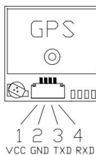
Figure 2: Pin Assignment
