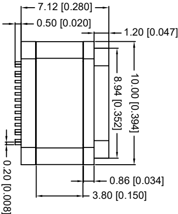
RECOMMENDED SCHEMATIC DRAWING OF CONNECTOR MATCH CHASSIS
